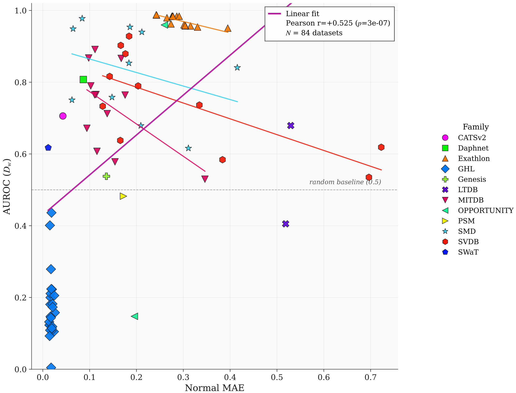
Forecast MAE vs anomaly-detection AUROC ( N = 84 datasets)
