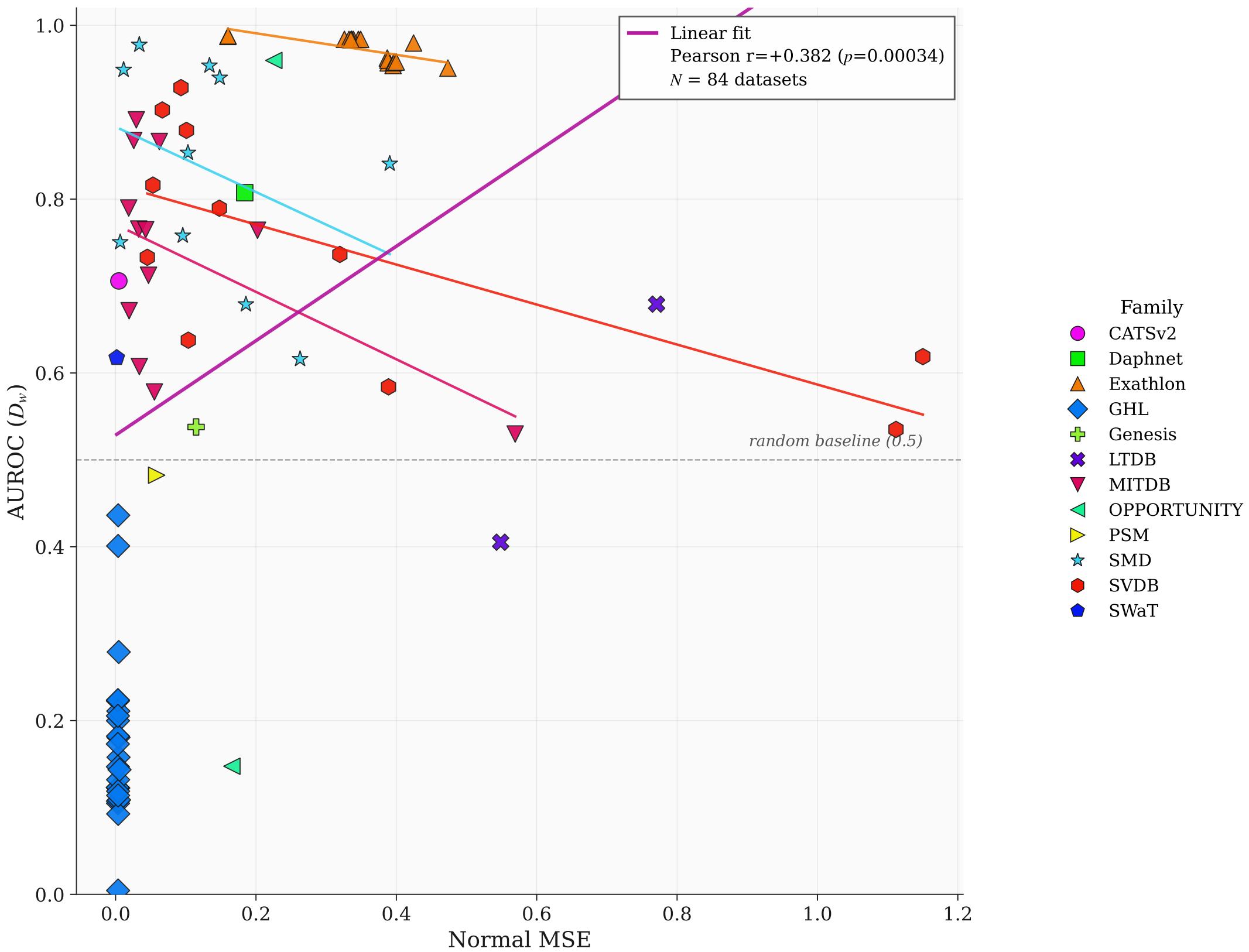
Forecast MSE vs anomaly-detection AUROC ( N = 84 datasets)
