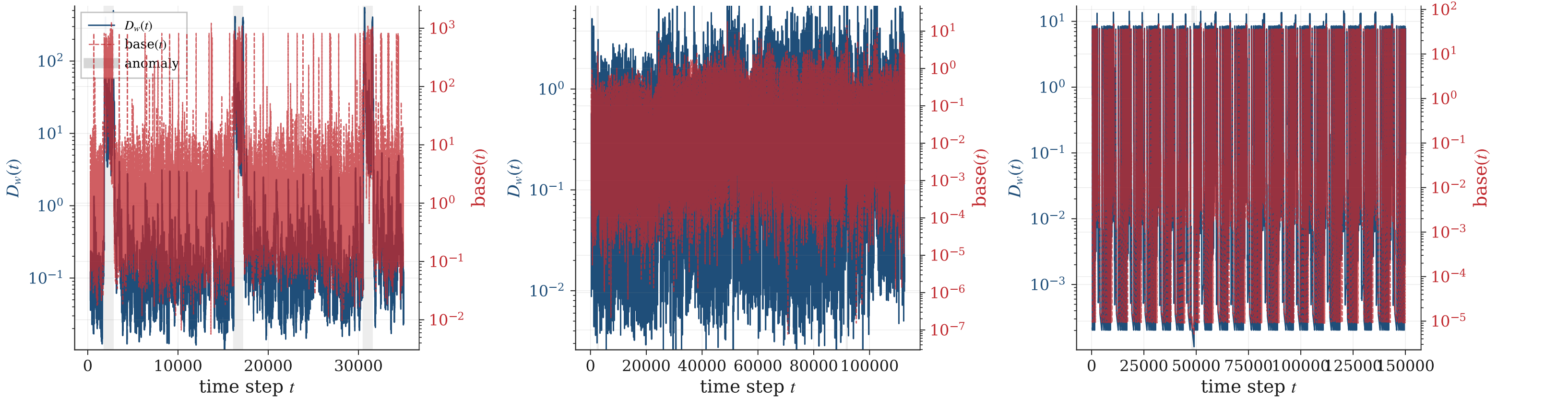
(a) Best: Exathlon_id_8 \text{AUROC}_{D_w} = 0.988 , \text{AUROC}_{\text{base}} = 0.994 (b) Median: MITDB_id_10 \text{AUROC}_{D_w} = 0.712 , \text{AUROC}_{\text{base}} = 0.676 (c) Worst: GHL_id_21 \text{AUROC}_{D_w} = 0.004 , \text{AUROC}_{\text{base}} = 0.017
