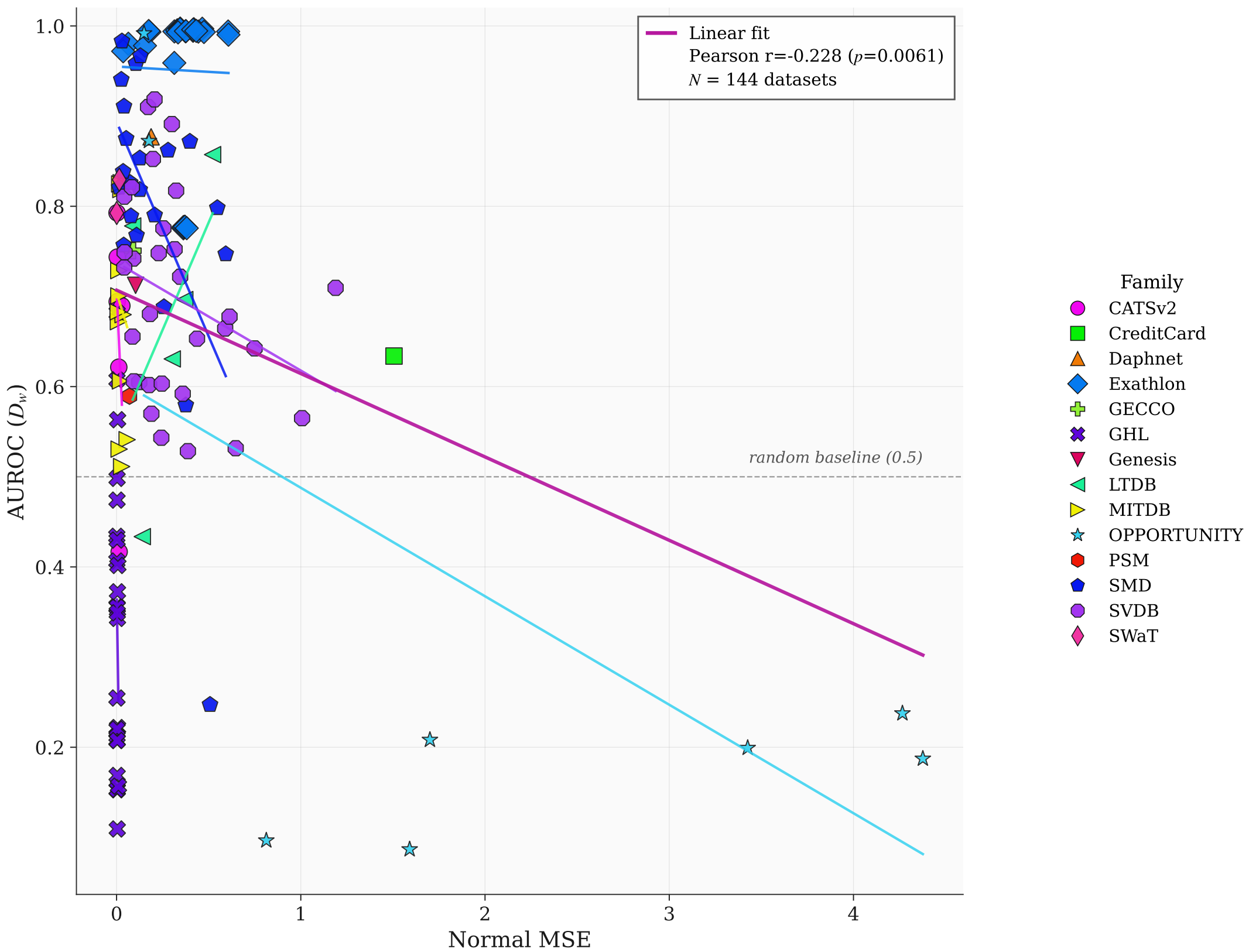
Forecast MSE vs anomaly-detection AUROC ( N = 144 datasets)
