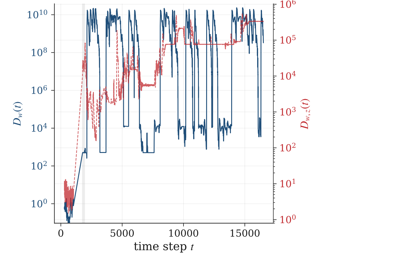
(c) Worst: OPPORTUNITY_id_6 AUROC _{D_w} = 0.087, AUROC _{D_{w,z}} = 0.237
