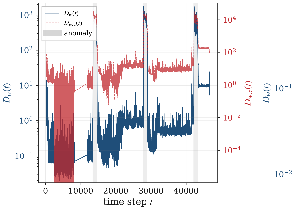
(a) Best: Exathlon_id_10 AUROC _{D_w} = 0.997, AUROC _{D_{w,z}} = 0.997
