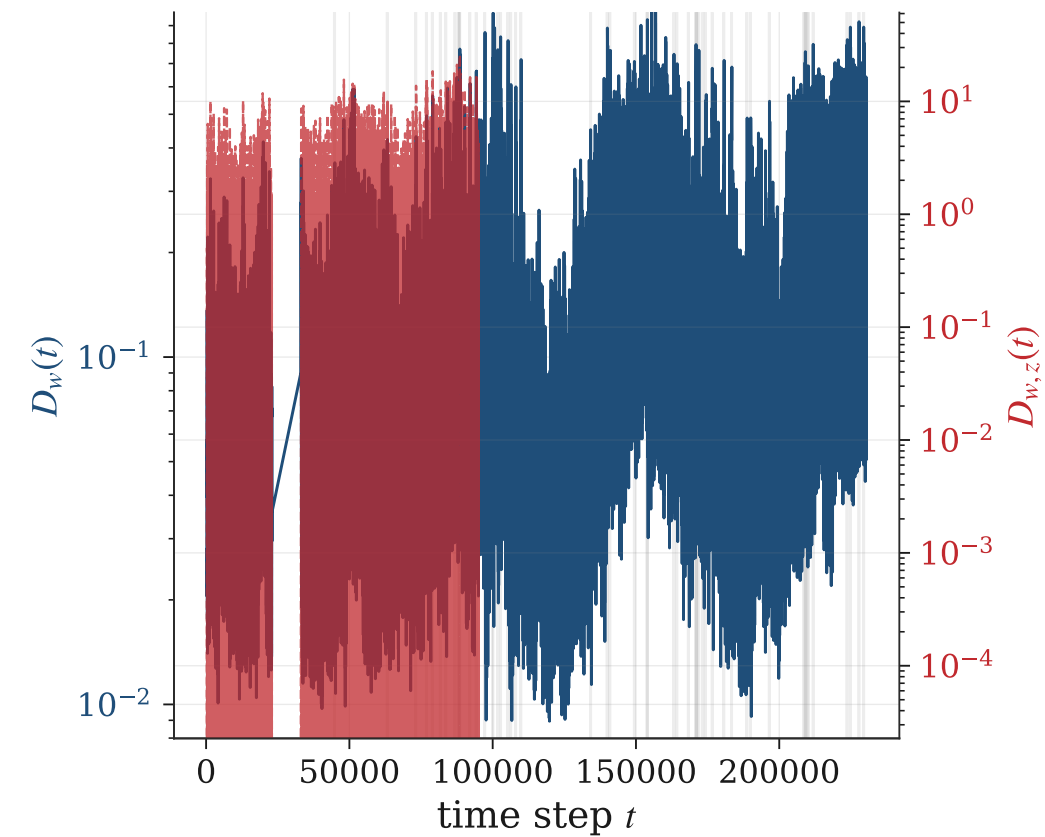
(b) Median: SVDB_id_24 AUROC _{D_w} = 0.732, AUROC _{D_{w,z}} = 0.731
