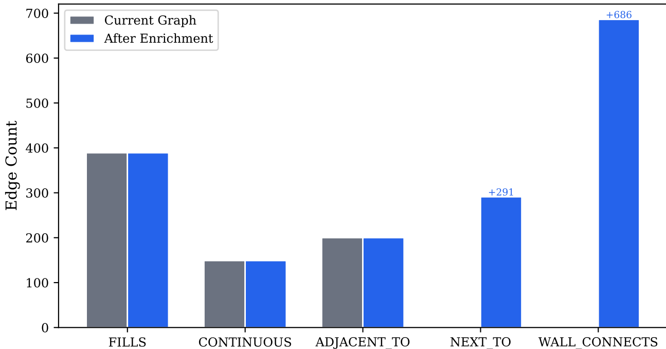
Graph Edges — Before vs After Enrichment
