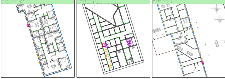
Figure 6.4. OpenCV-based contour visualization sample. Red circle is the target and yellow circle is the valid counts, which able to extract position_context such as "3rd of 17 openings".
