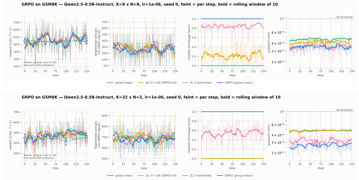
Figure 3: Seed 0 of the corrected sweep at K=8, N=8 (top) and K=32, N=2 (bottom). Reward and degenerate-group panels overlap; the shrinkage panel separates the arms, and at N=2 js_fixed lies on global ’s zero line for the whole run. No gradient norm reaches the clip threshold. Faint lines are per-step values, bold a rolling window — median for the gradient norm.
