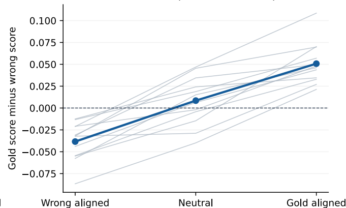
MiniLM cross-encoder (raw logit)
