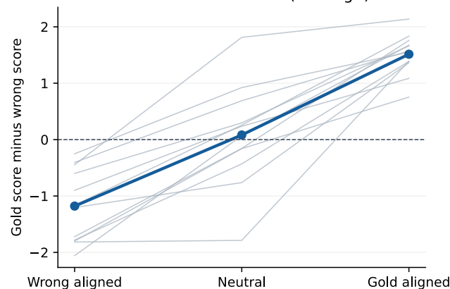
MiniLM cross-encoder (raw logit)
