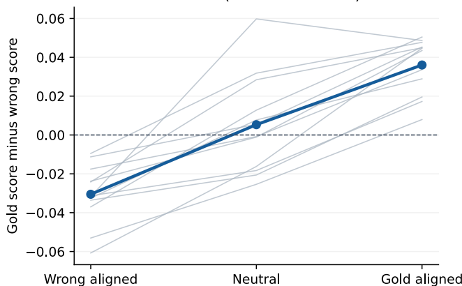
E5-small (unscaled cosine)
