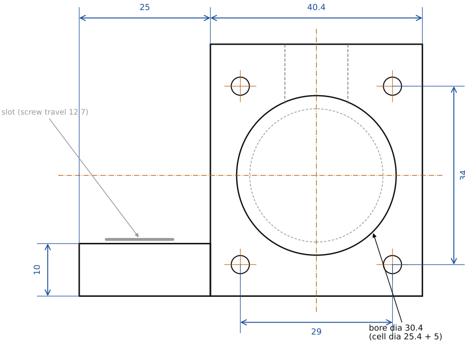
END VIEW (+x end face)
