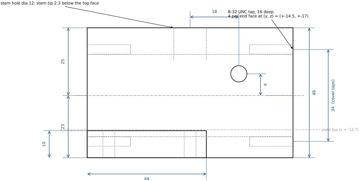
SIDE VIEW (from -y, the shoulder side)
