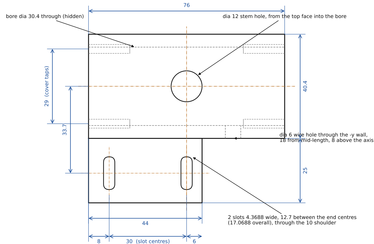
TOP VIEW (looking down -z)
