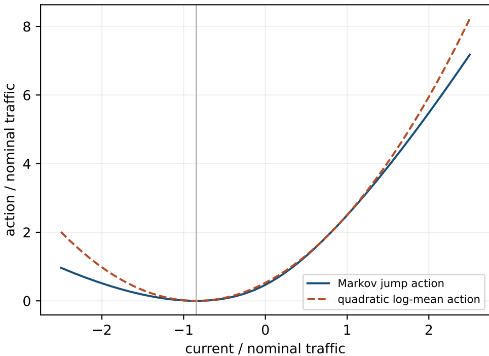
Same minimum, different fluctuation cost
