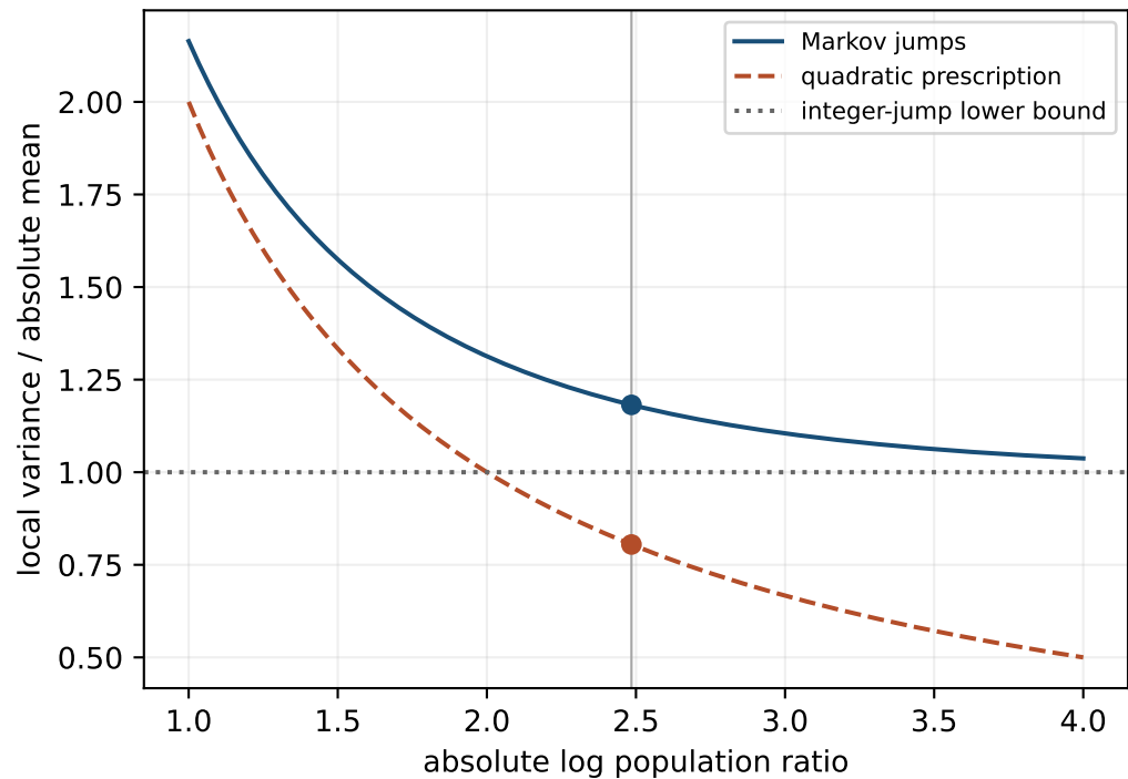
A microscopic counting consistency test
