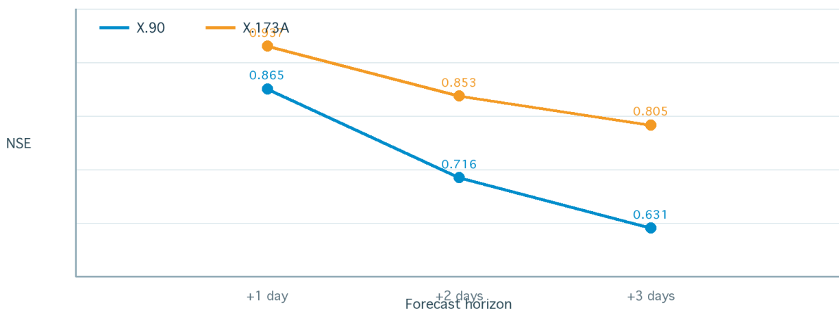
Temporal-test performance by forecast horizon
