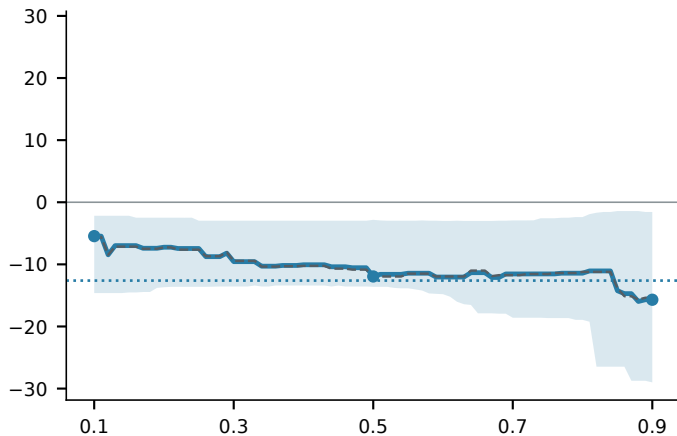
(c) Cool days
