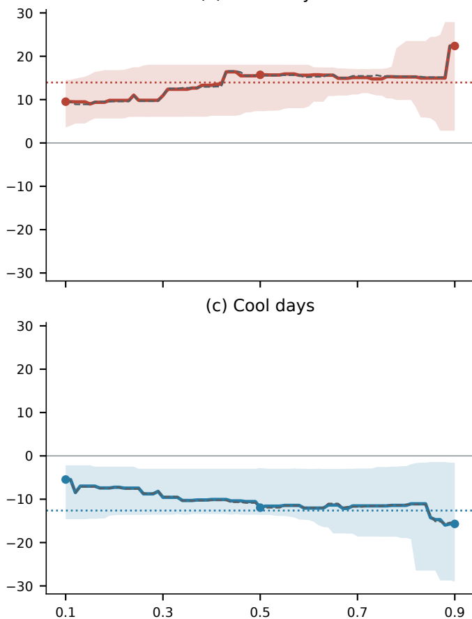
(a) Warm days
