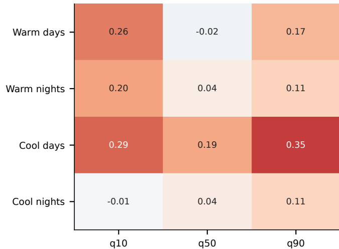
(a) Moran's I
