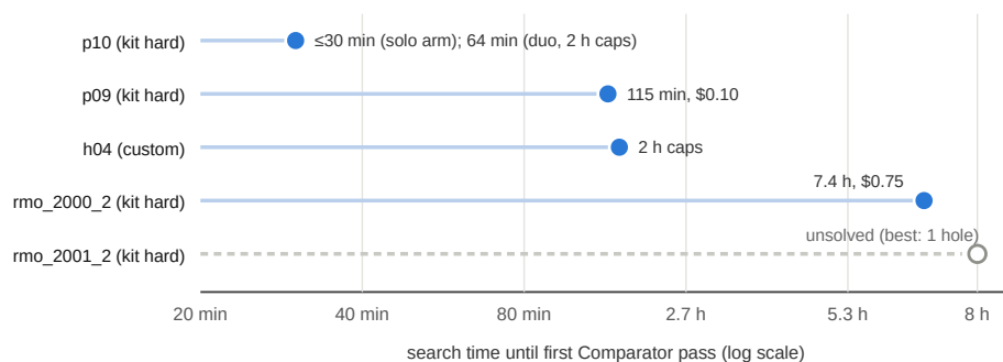
Figure 3: Time until each hard problem first passed the Comparator (hollow marker = unsolved). p10 falls within short caps; every other solve in this tier came at a multi-hour horizon under decomposition; h04 had resisted ~19 short-window configurations.
