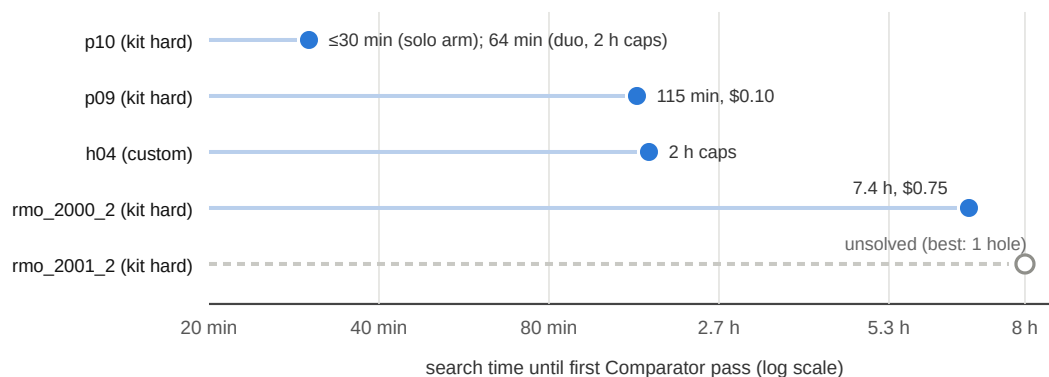
Figure 3: Time until each hard problem first passed the Comparator (hollow marker = still unsolved). p10 falls within short caps under the controller; every other solved instance in this tier fell only at a multi-hour horizon under S4 decomposition. For context, the dev-16 aggregate did not change when the short window was doubled from 20 to 40 minutes (11–13 → 11, within the noise band). h04 is a custom problem that had not been solved by any of ~19 short-window configurations before the 2-hour run.
