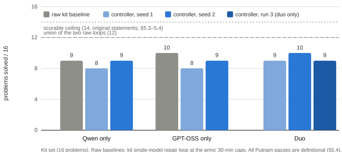
Figure 2: Cap-matched regime: same controller, model set switched, identical 30-minute caps, two seeds per arm plus a third duo run. Raw bars: the kit's single-model repair loop at the same 30-minute caps. Putnam passes in every bar use the definitional route of §5.4.
