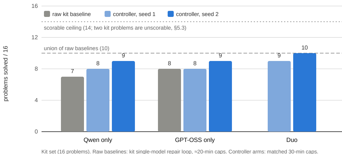
Figure 2: Cap-matched regime: same controller, model set switched, identical 30-minute caps, two seeds per arm. Raw kit baselines ( \approx 20 -minute caps) are per-model floors, not scaffold-isolating controls.
