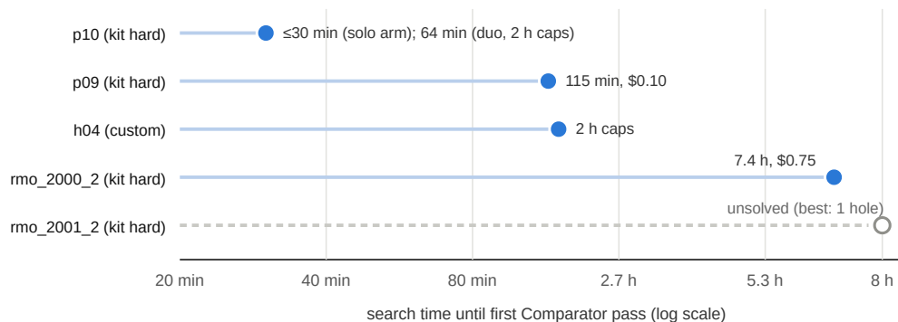
Figure 3: Time until each hard problem first passed the Comparator (hollow marker = still unsolved). p10 falls within short caps (a controller arm; once, the raw GPT-OSS loop); every other solved instance in this tier fell only at a multi-hour horizon under S4 decomposition. The dev-16 aggregate did not change when the short window was doubled from 20 to 40 minutes (11–13 → 11, within the noise band). h04 is a custom problem unsolved by \sim 19 short-window configurations before the 2-hour run.
