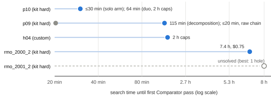
Figure 3: Time until each hard problem first passed the Comparator on the controller's decomposition path (blue; hollow marker = unsolved), with the earliest pass by any configuration in grey where it differs. p10 and, via the raw chain (§6.1), p09 fall within short caps; rmo_2000_2 and h04 came only at multi-hour horizons under decomposition; h04 had resisted ~19 short-window configurations.
