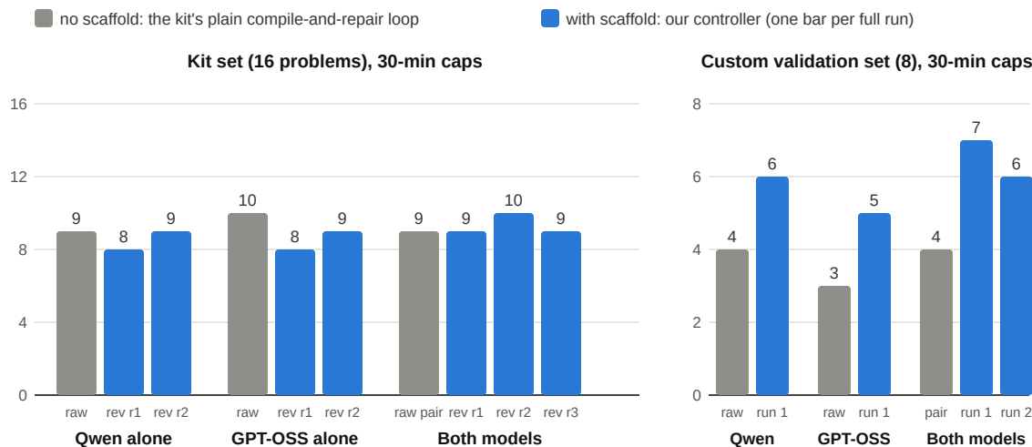
Figure 2: Scaffold effect at matched 30-minute caps. Grey: no scaffold, the kit's plain compile-and-repair loop run with the named model (for both models, two such loops in parallel; the first accepted proof wins). Blue: the same models inside our controller, one bar per full run (left: revisions r1, r2, r3 of §4; right: two runs under r4). Left, the kit's 16 problems: the scaffold ties the plain loops. Right, the eight custom validation problems (all arms under revision r4, §4): the scaffold adds two problems per model and two to three for both models; m03 and h03 were solved only with the scaffold.
