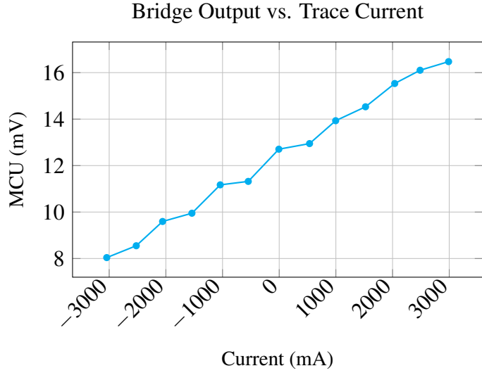
Figure 15: Plot of the shielded current sweep data detailed in Table 6.
