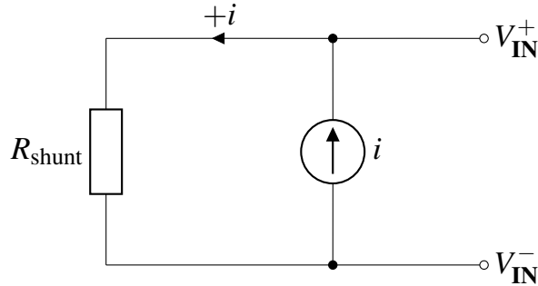
Figure 6: Field excitation circuit schematic and positive trace current convention ( +i ).
