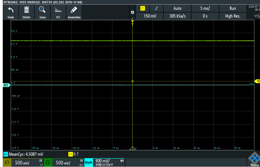
Figure 4: Isolated-board saturation characteristics
