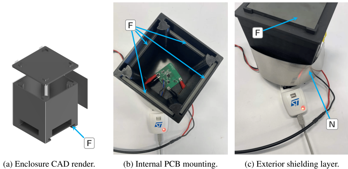
Figure 12: Development of the magnetic shielding enclosure. (a) The 3D-printed chassis. (b) The integrated sensor board mounted inside. (c) The assembled test configuration wrapped in shielding. Annotations indicate the placement of ferrite plates (F) and flexible nanocrystalline shielding (N).
