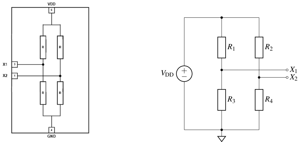
(a) CT100 internal Wheatstone-bridge.
