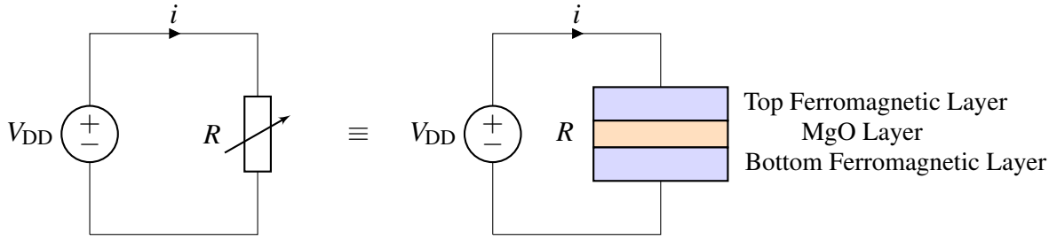
Figure 1: Equivalent electrical circuit model equating a standard variable resistor (left) to the physical three-layer Magnetic Tunnel Junction stack structure (right).
