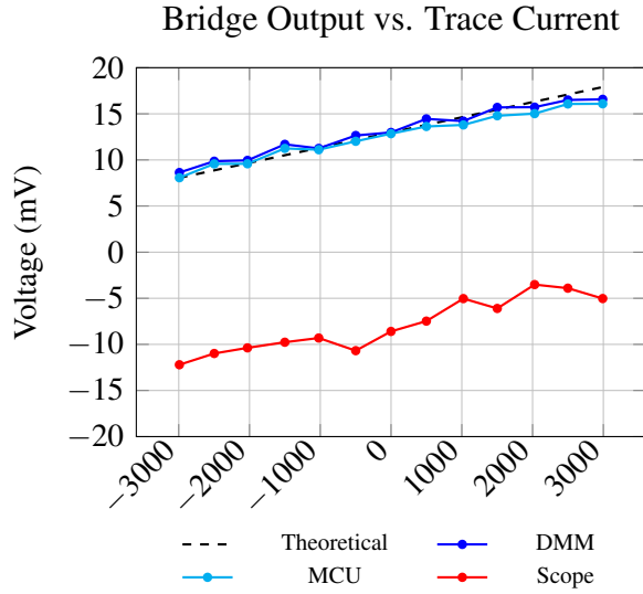
Figure 9: Voltage cross-validation during the non-irradiated, unshielded current sweep. The dashed line shows the theoretical CT100 response.
