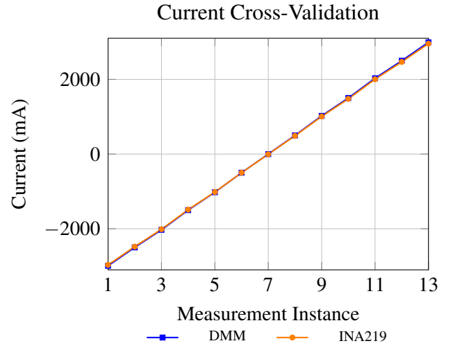
Figure 10: Current cross-validation across the 13-point sweep.
