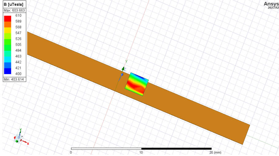
Figure 7: Ansys near-field simulation of the current trace.
