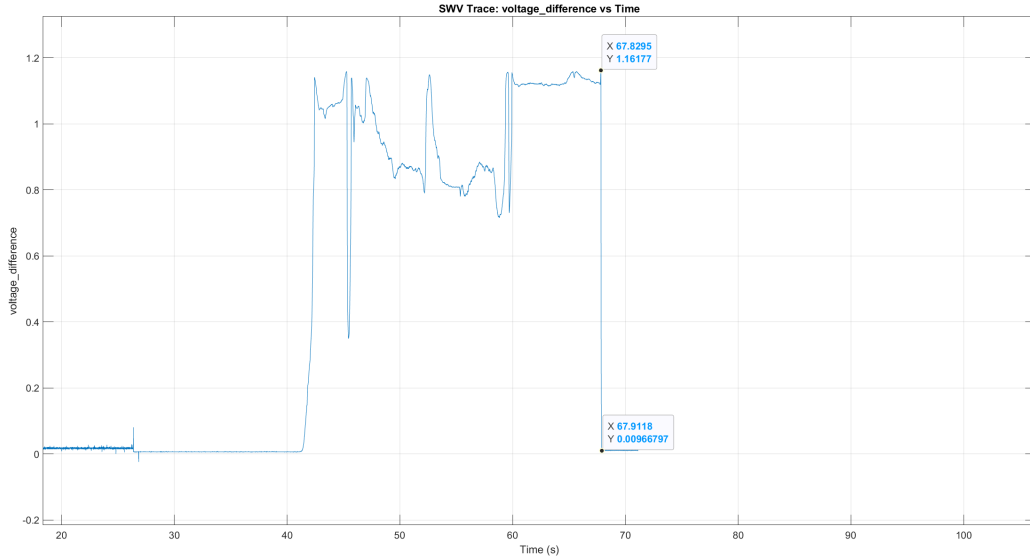
Figure 8: Measured saturation recovery response on the integrated board (SWV trace, logged and plotted in MATLAB).
