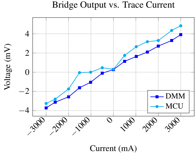
Figure 11: Plot of irradiated DMM and MCU sweeps detailed in Table 3.
