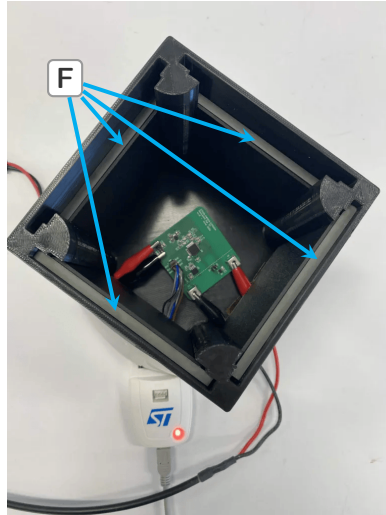
(b) Internal PCB mounting.
