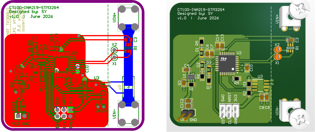
Figure 5: Integrated board layout (left) and rendered assembly view (right).
