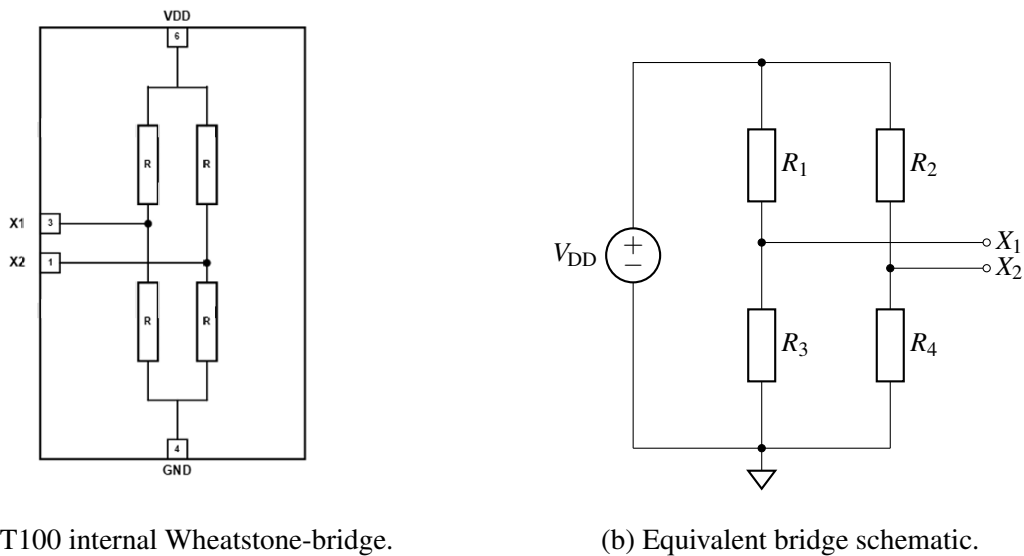
Figure 2: Internal CT100 IC pin configuration alongside its labeled equivalent electrical schematic.
