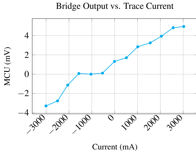
Figure 14: Plot of the irradiated, shielded current sweep data detailed in Table 6.
