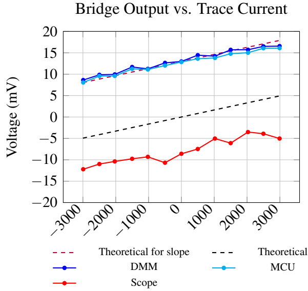
Figure 9: Voltage cross-validation during the non-irradiated, unshielded current sweep. The dashed line shows the theoretical CT100 response.
