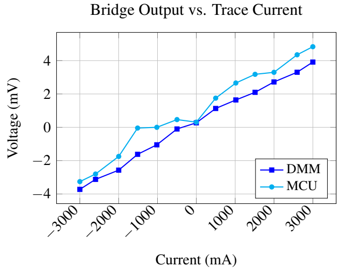
Figure 11: Plot of irradiated DMM and MCU sweeps detailed in Table 4.
