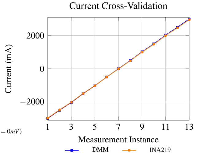
Figure 10: Current cross-validation across the 13-point sweep.
