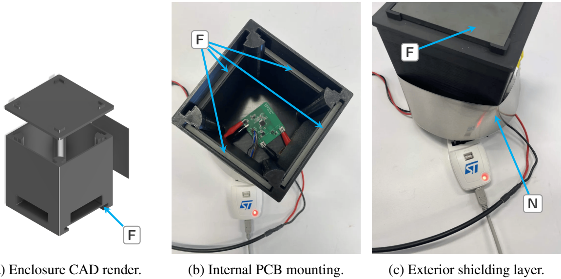
Figure 14: Development of the magnetic shielding enclosure. (a) The 3D-printed chassis. (b) The integrated sensor board mounted inside. (c) The assembled test configuration wrapped in shielding. Annotations indicate the placement of ferrite plates (F) and flexible nanocrystalline shielding (N).
