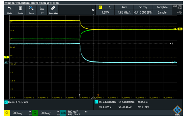
(b) Sample 3: Positive Saturation Recovery
