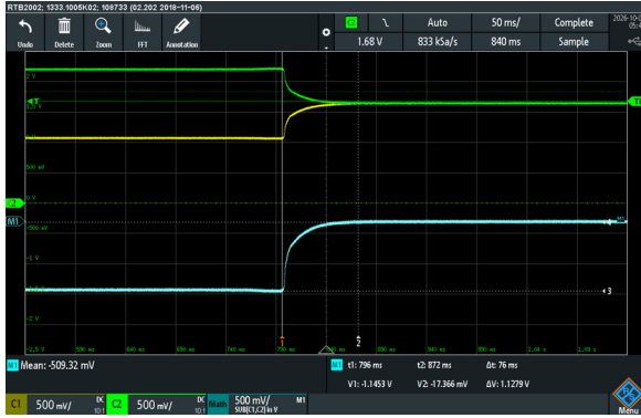
(c) Sample 2: Negative Saturation Recovery
