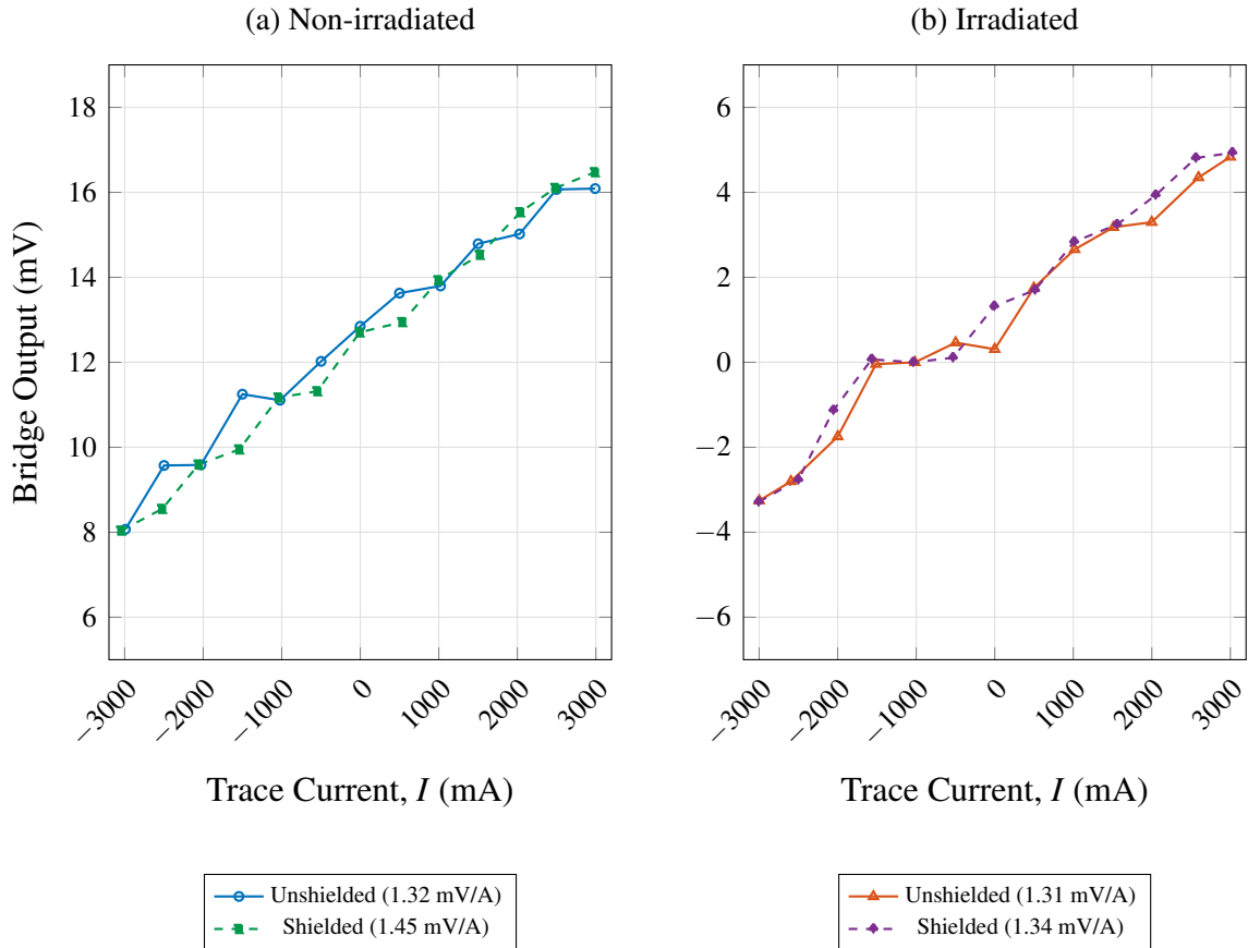
Figure 15: Shielded vs. unshielded current sweeps (MCU readings) for (a) the non-irradiated and (b) the irradiated sample.
