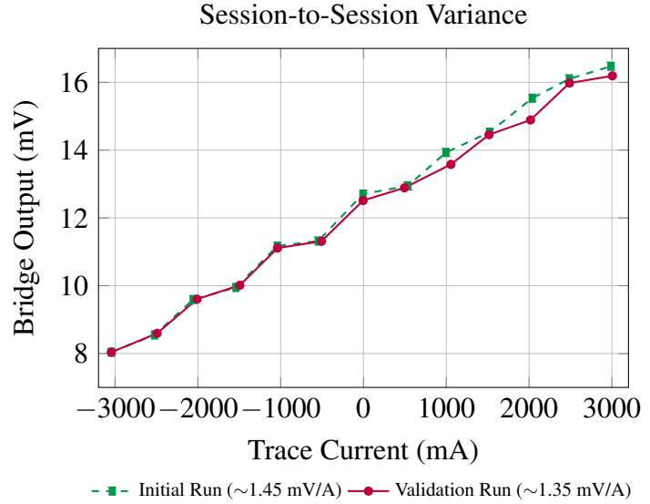
Figure 16: Plots of two discrete testing sessions on the same shielded, non-irradiated board.
