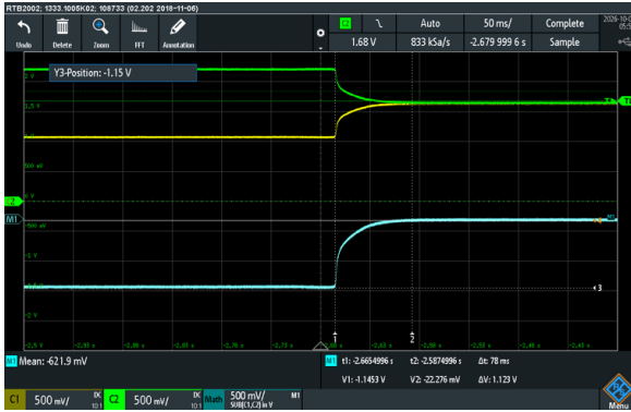
(c) Sample 4: Negative Saturation Recovery
