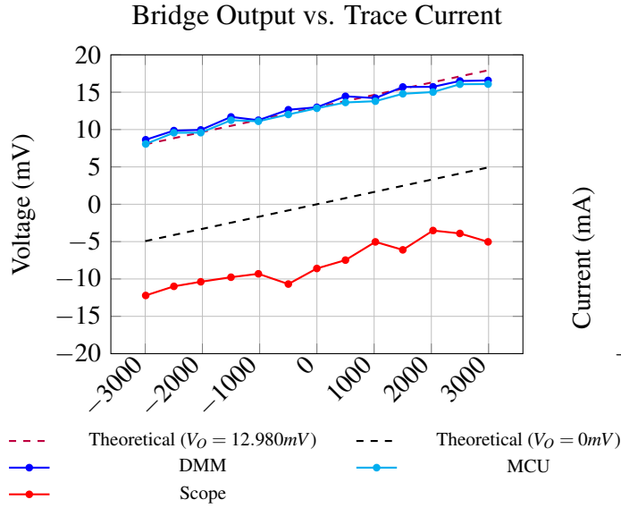
Figure 9: Voltage cross-validation during the non-irradiated, unshielded current sweep. The dashed lines shows the theoretical CT100 responses.
