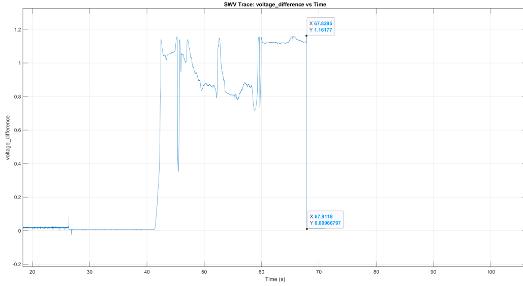
Figure 13: Measured saturation recovery response on the integrated board (SWV trace, logged and plotted in MATLAB).
