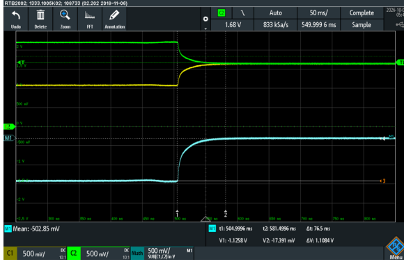
(a) Sample 1: Negative Saturation Recovery
