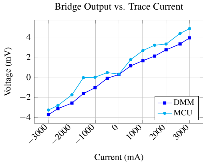
Figure 13: Plot of irradiated DMM and MCU sweeps detailed in Table 5.
