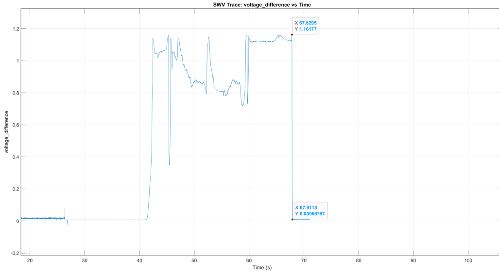
Figure 14: Measured saturation recovery response on the integrated board (SWV trace, logged and plotted in MATLAB).
