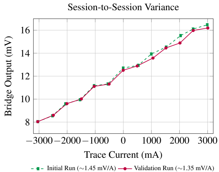
Figure 17: Plots of two discrete testing sessions on the same shielded, non-irradiated board.
