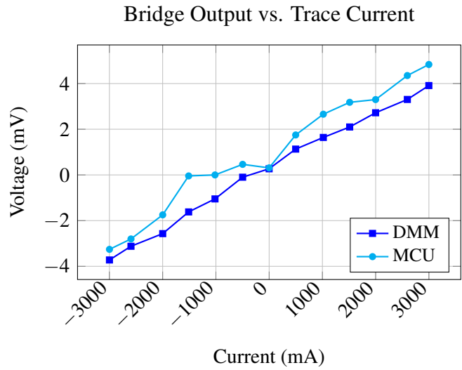
Figure 13: Plot of irradiated DMM and MCU sweeps detailed in Table 6.
