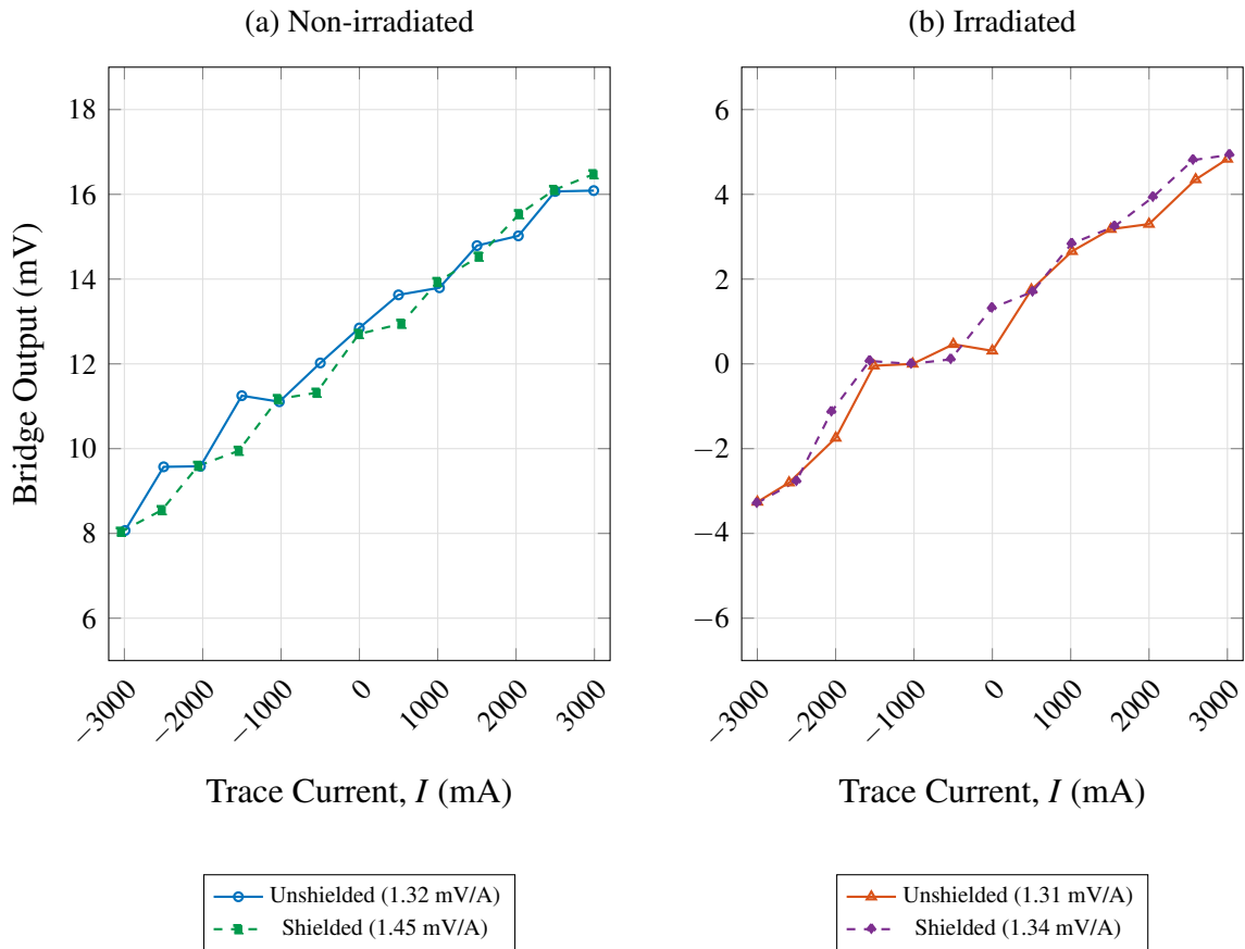
Figure 16: Shielded vs. unshielded current sweeps (MCU readings) for (a) the non-irradiated and (b) the irradiated sample.
