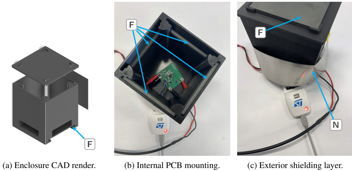
Figure 15: Development of the magnetic shielding enclosure. (a) The 3D-printed chassis. (b) The integrated sensor board mounted inside. (c) The assembled test configuration wrapped in shielding. Annotations indicate the placement of ferrite plates (F) and flexible nanocrystalline shielding (N).
