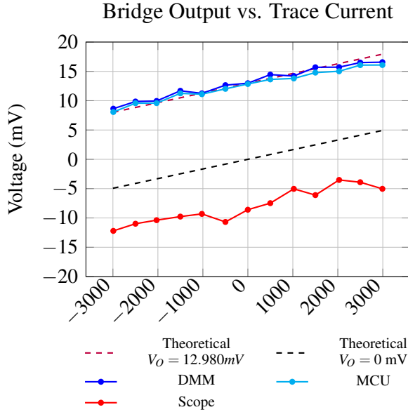
Figure 9: Voltage cross-validation during the non-irradiated, unshielded current sweep. The dashed lines shows the theoretical CT100 responses.
