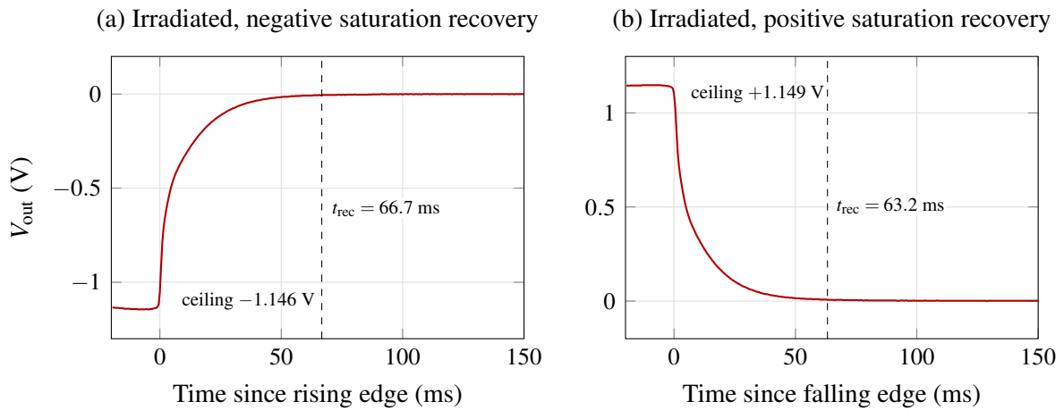
Figure 14: Irradiated Saturation recovery on the integrated board after the magnet is removed, for both field directions.
