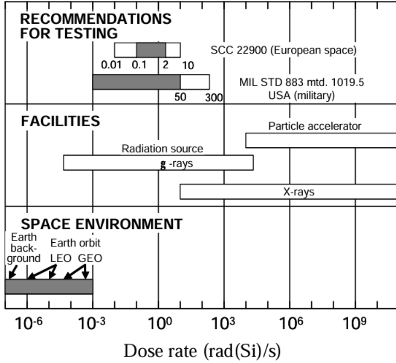
Figure 11: Comparison of the dose rates found in the radiation environments and the rates used in the testing of components for tolerance.
