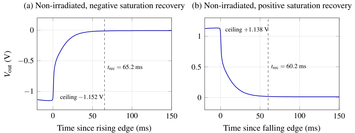
Figure 8: Non-Irradiated Saturation recovery on the integrated board after the magnet is removed, for both field directions.
