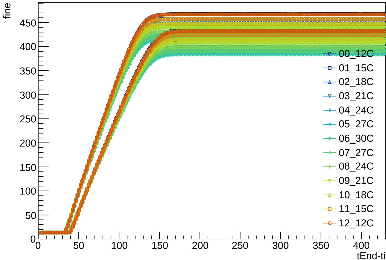
[pFine] chip00&01_chan00_tac0
