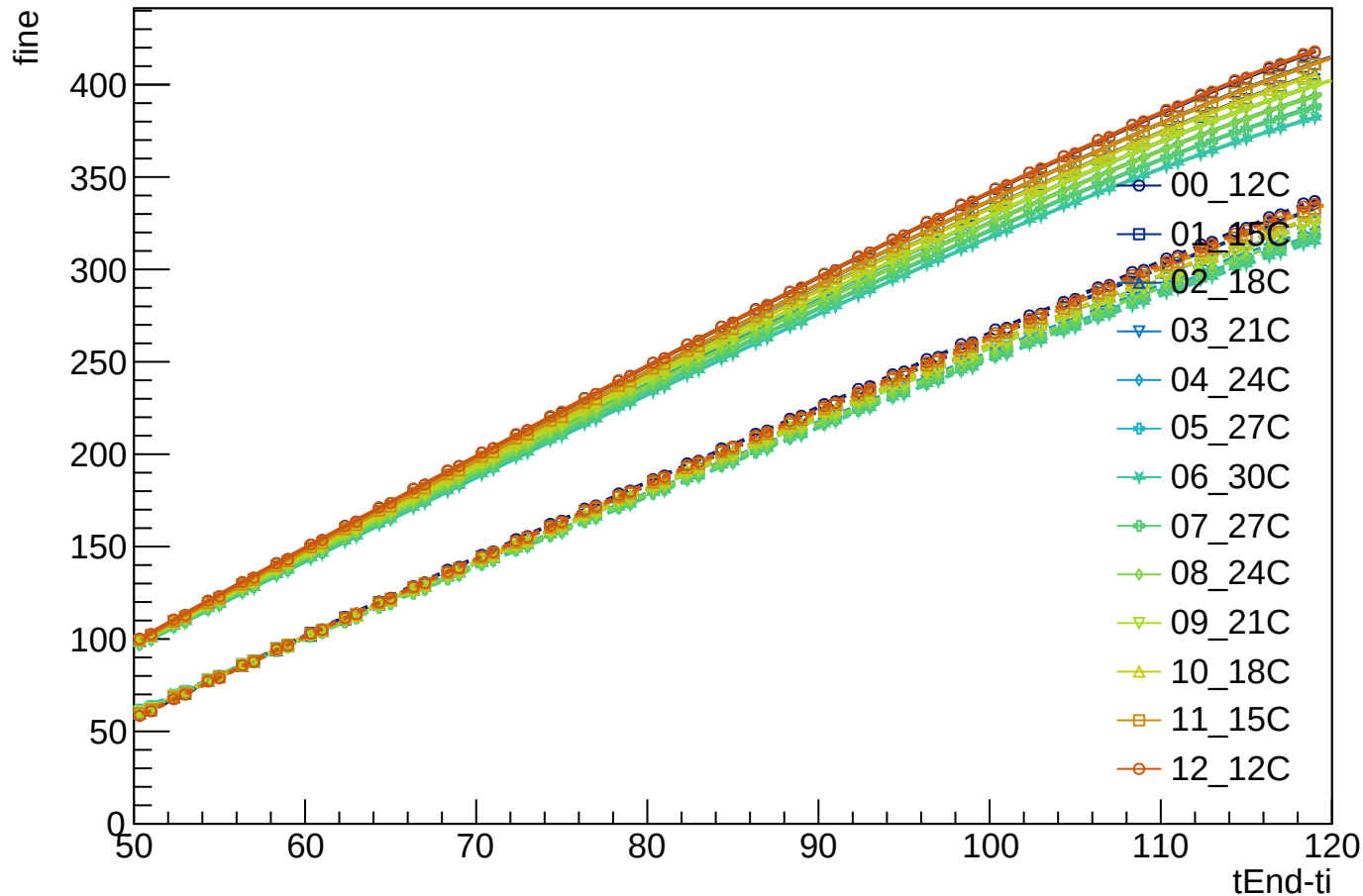
[pFine] chip00&01_chan00_tac0
