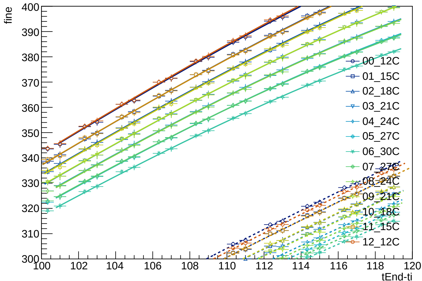
[pFine] chip00&01_chan00_tac0
