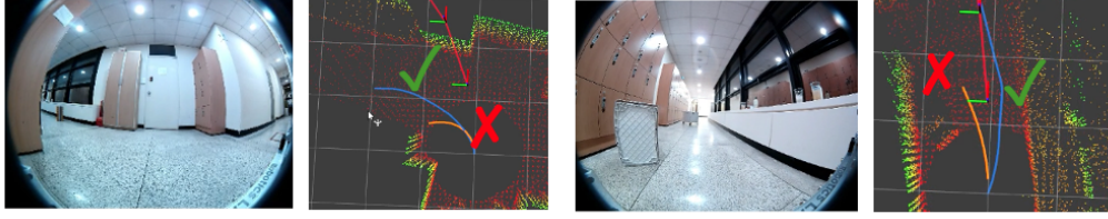
Figure 1: PathLift in action. The raw NoMaD output (red) is the unitless prior. Lifted by a constant scalar baseline (orange, \times ), the trajectory drives the robot into structural obstacles; lifted by PathLift (blue, \checkmark ), it routes around them. Each pair shows the fisheye RGB and the corresponding BEV with occupied cells (black) and depth points (brown).
