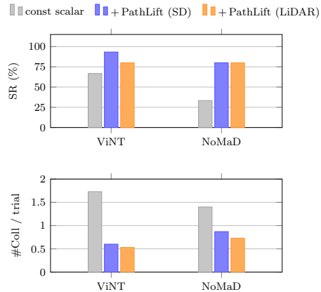
Figure 5: Results on different depth sources: success rate (top) and collisions per trial (bottom).
