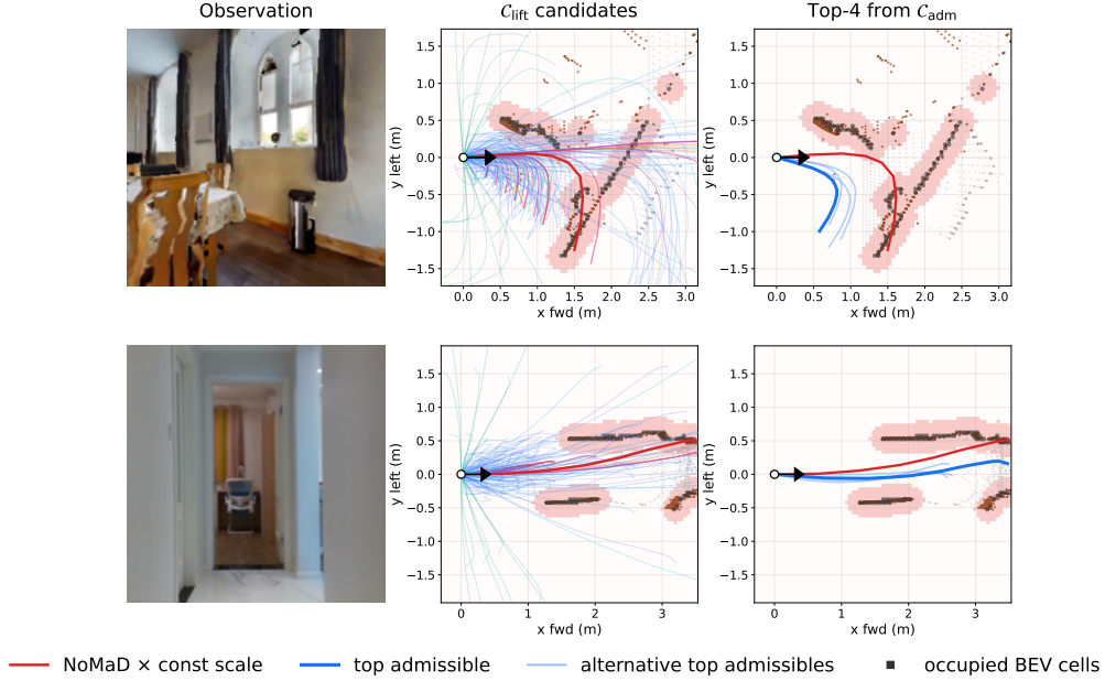
Figure 3: Supervision target on Habitat (top) and OpenLORIS (bottom). Col. 1: camera RGB. Col. 2: all candidates in \mathcal{C}_{\text{lift}}(\hat{p}) from the NoMaD prior (faded). Col. 3: four lowest-ADE admissibles; supervision target in solid blue. The NoMaD \times const scale (red) and occupied BEV cells (black) overlaid in both BEV columns.
