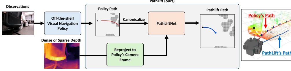
Figure 2: PathLift inference pipeline. An off-the-shelf visual-navigation policy emits a unitless policy path; the canonicalized prior and a depth observation (RGB-D, stereo, or projected LiDAR) reprojected into the policy’s camera frame feed PathLiftNet, which outputs a metric trajectory in body coordinates.
