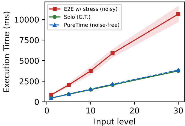
face-detect+sentiment (#faces) PureTime↔Solo median err 2.6%
