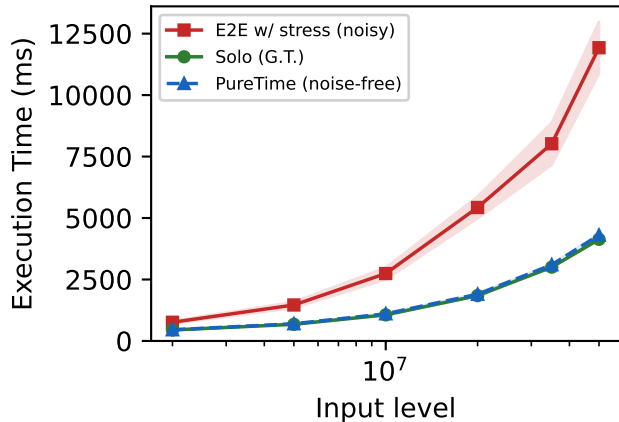
float (sqrt/sin/cos, iters) PureTime↔Solo median err 3.2%
