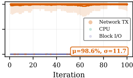
Injected: Network TX
