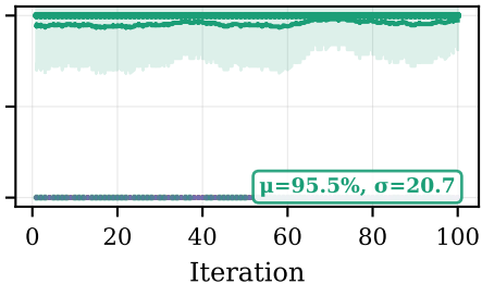
Injected: CPU
