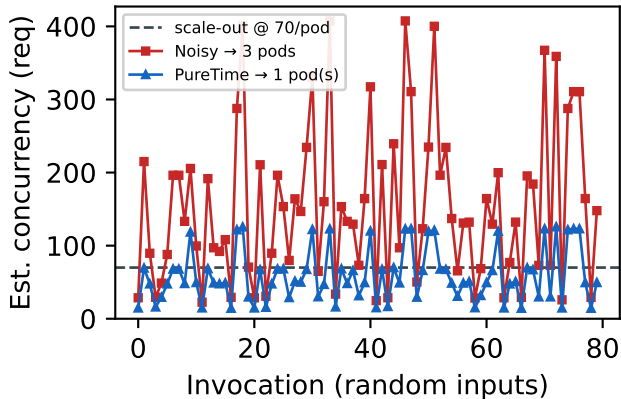
Knative KPA (Little's Law, concurrency= \lambda \cdot T )
