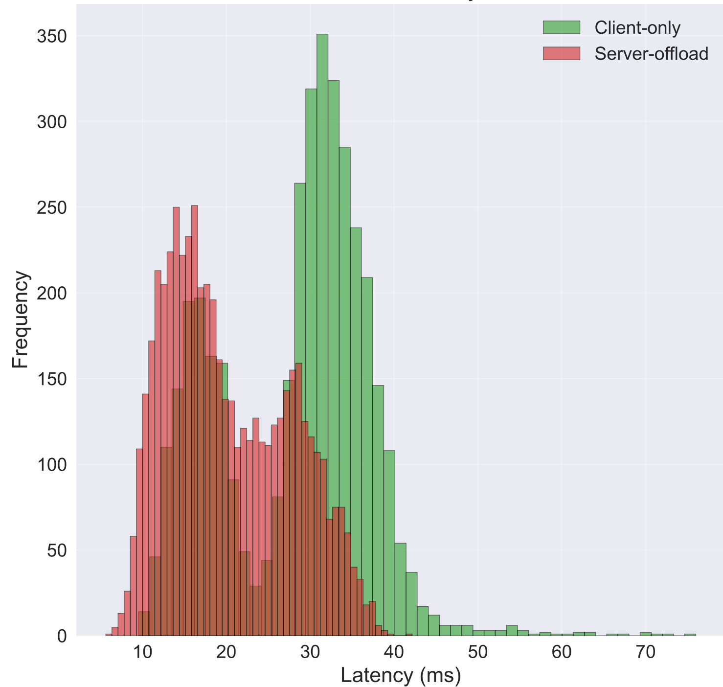
XREAL Interaction Latency Distribution
