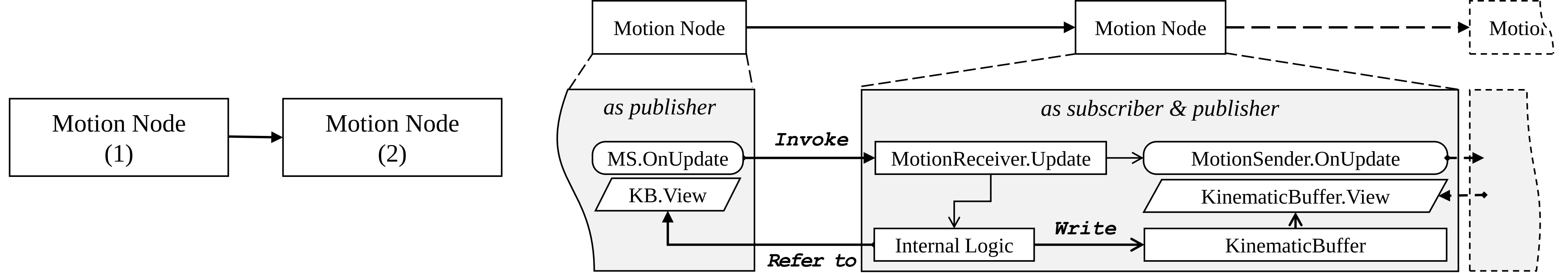
(a) Motion Node for Composition
