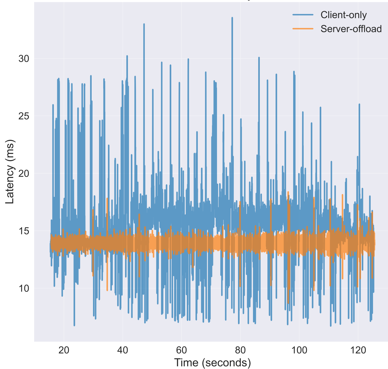
Quest Interaction Latency Over Time
