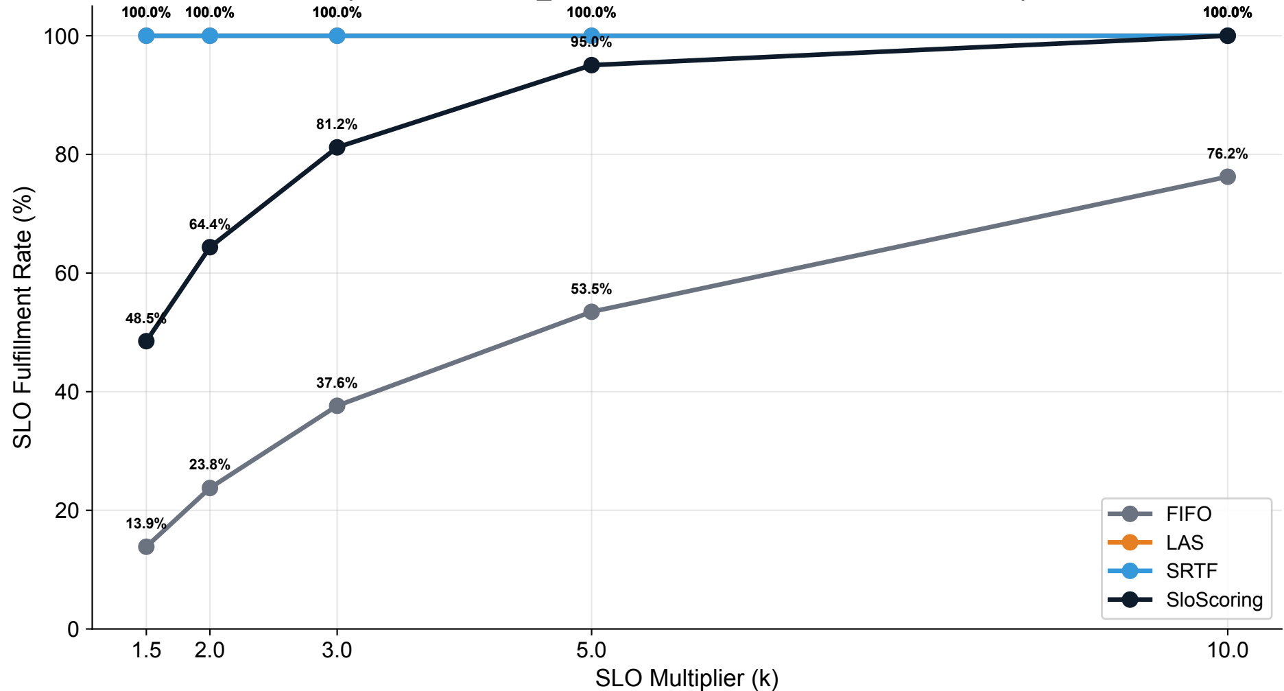
SLO Fulfillment Rate by Scheduler (SLO = k \times \text{ideal\_duration} , Alibaba GenAI Trace, Load=8)
