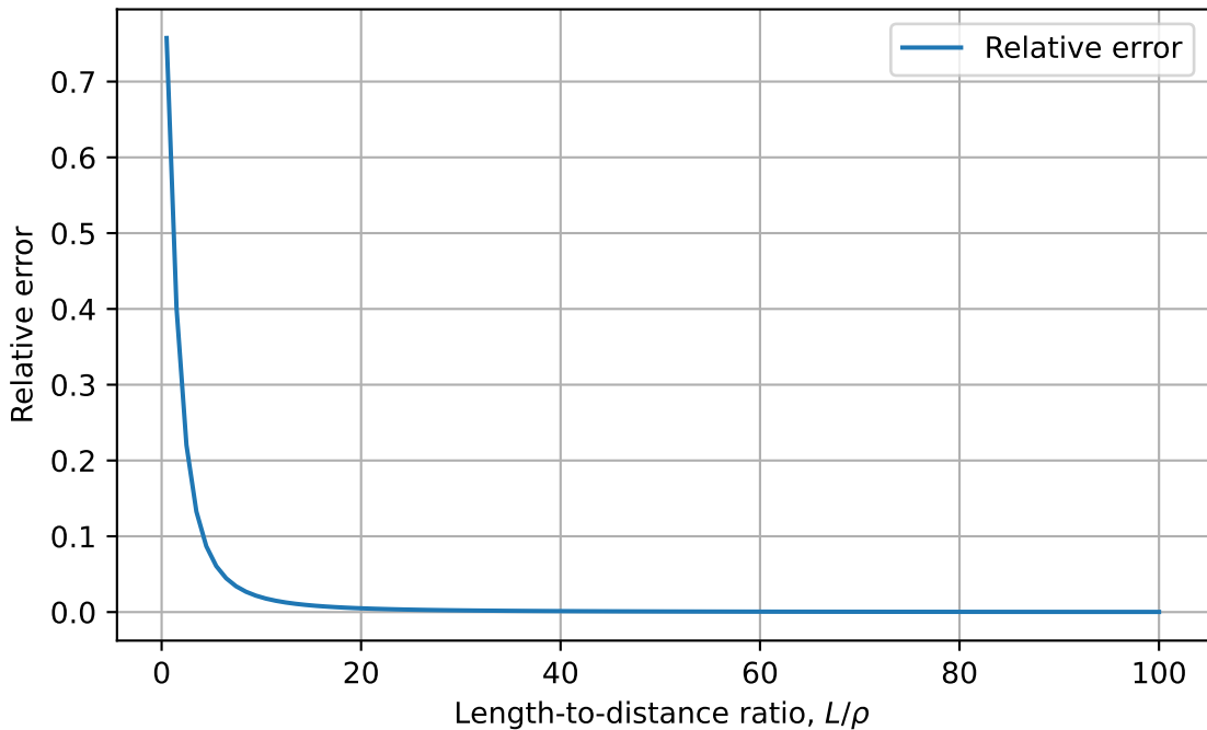
Convergence of a Finite Straight Wire to the Infinite-Wire Limit
