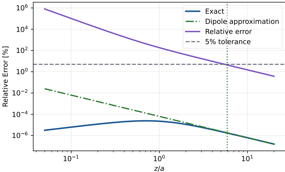
Accuracy of the Magnetic Dipole Approximation
