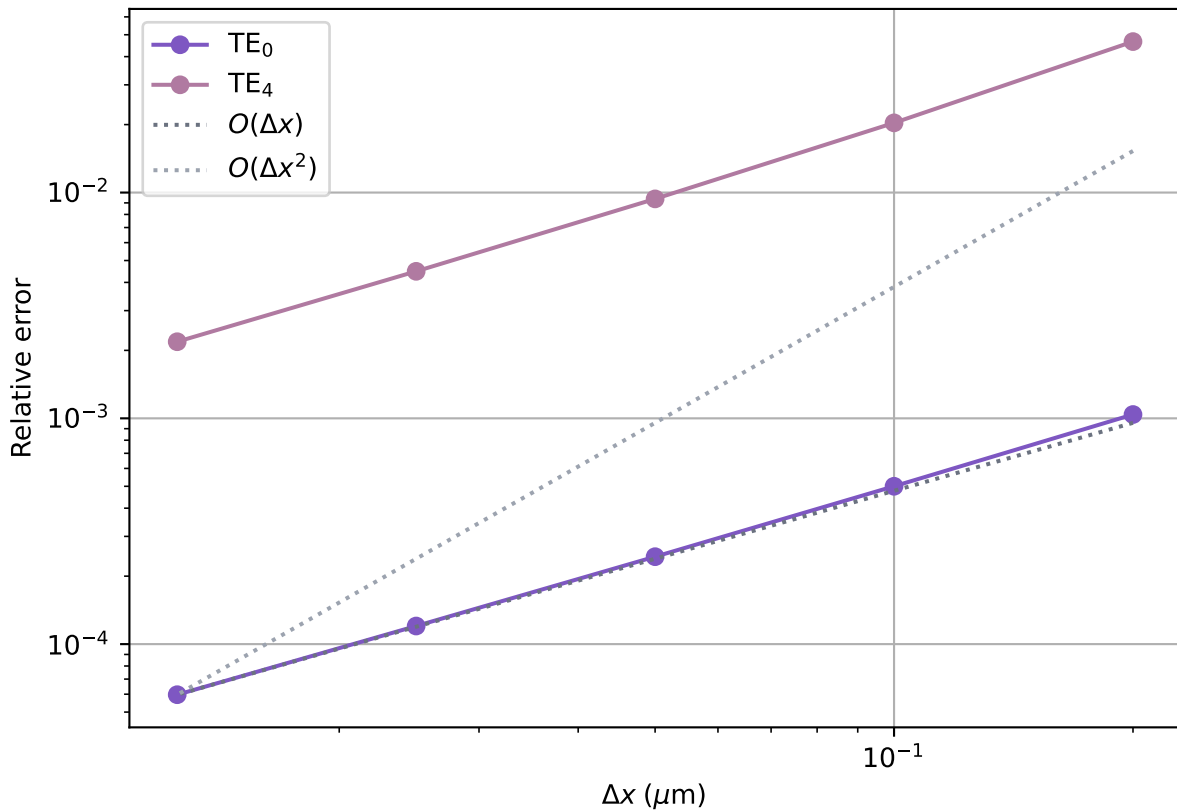
Grid Convergence of TE 0 and TE 4 Modes
