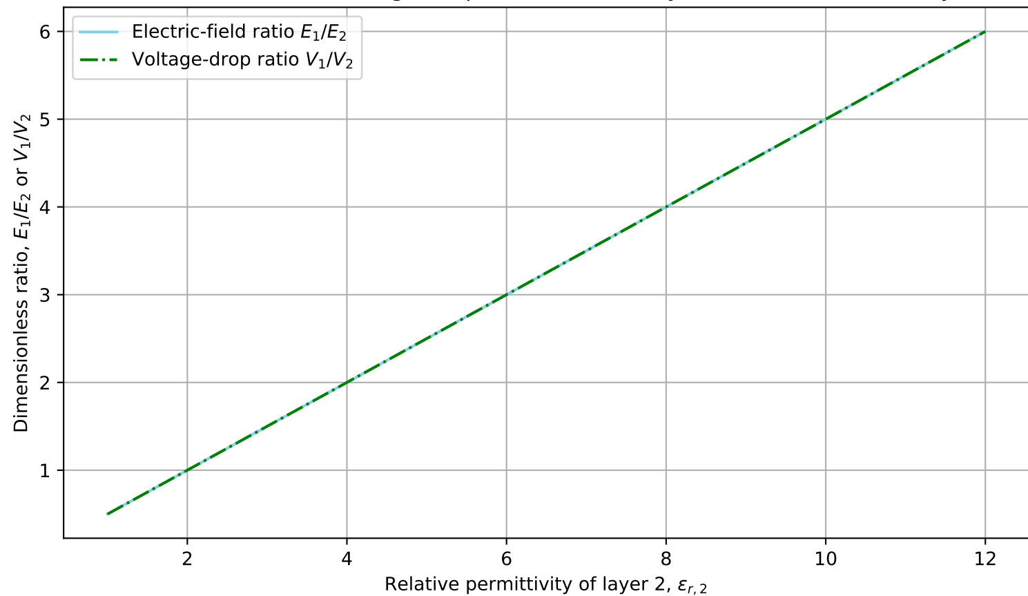
Electric-Field and Voltage-Drop Ratios versus Layer-2 Relative Permittivity
