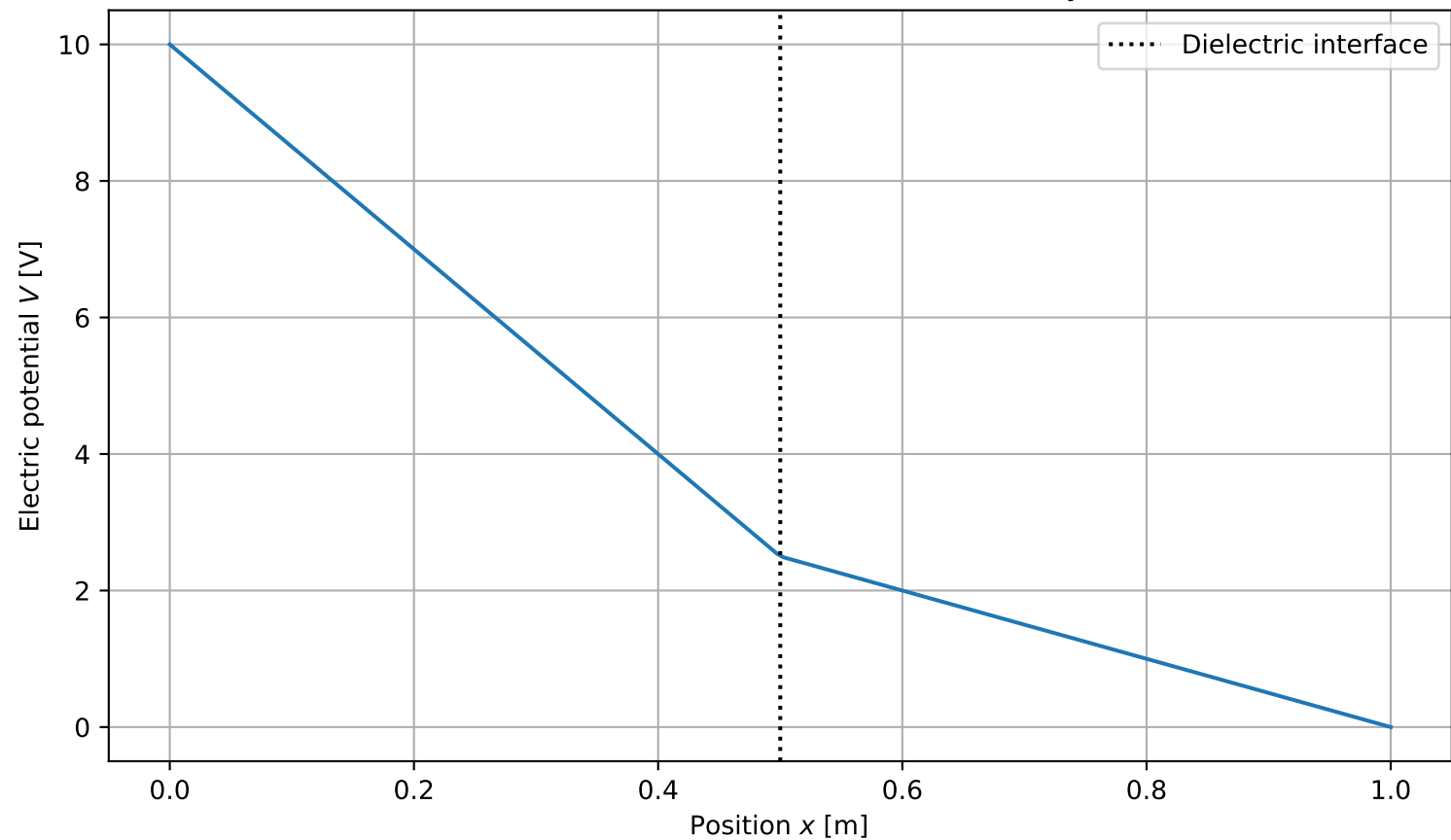
Electric Potential Across the Dielectric Layers
