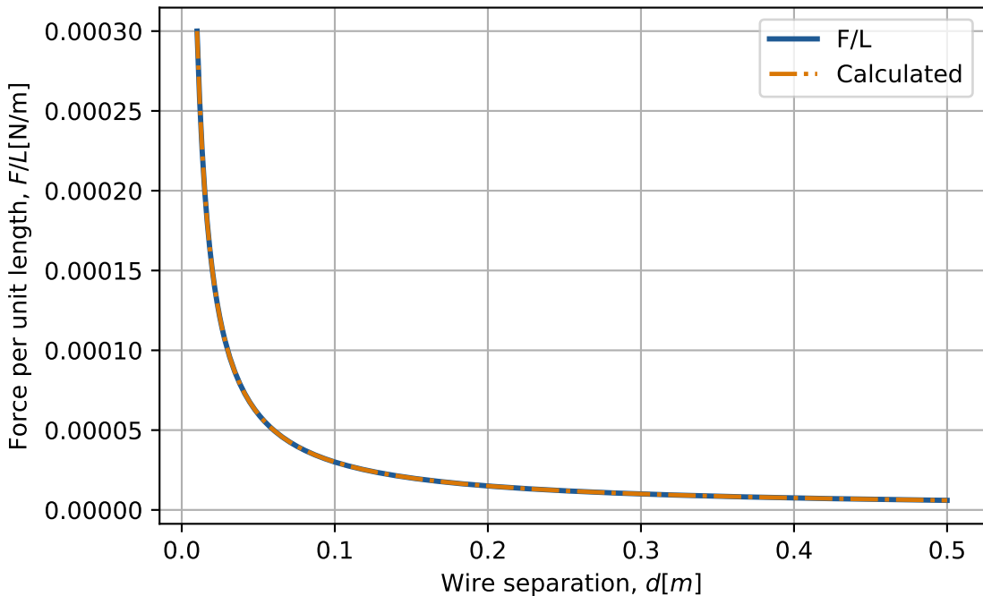
Magnetic Force per Unit Length versus Wire Separation
