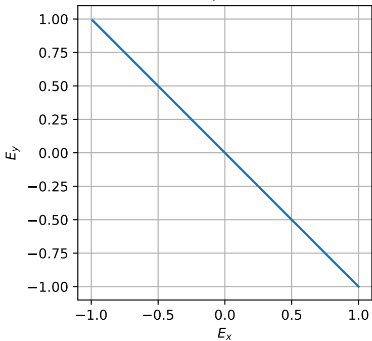
\Delta\phi = \pi
