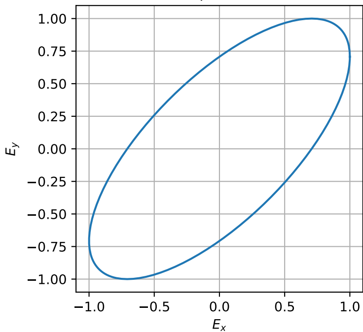
\Delta\phi = \pi/4
