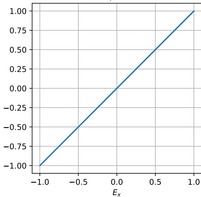
\Delta\phi = 0
