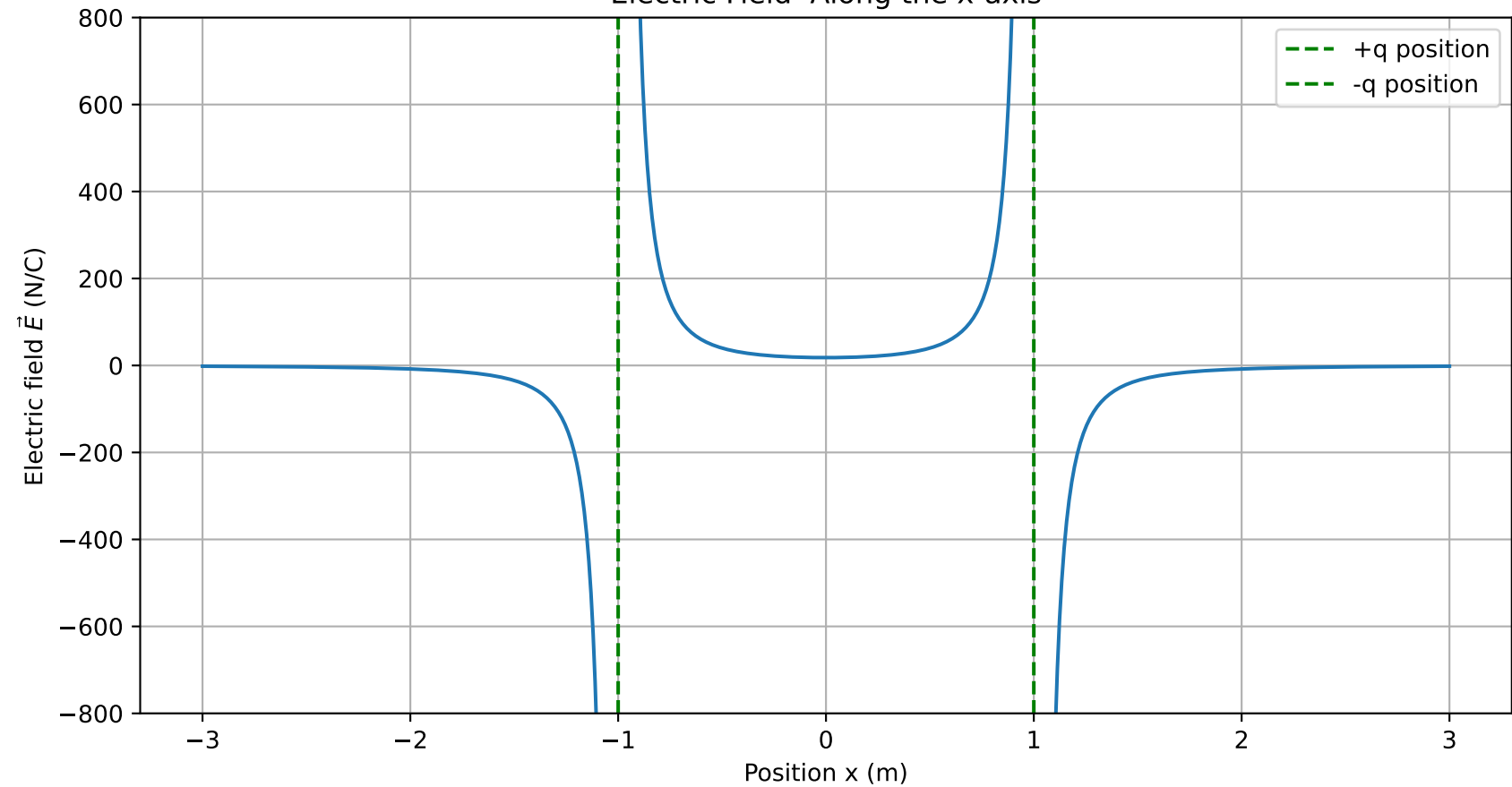
Electric Field Along the x-axis
