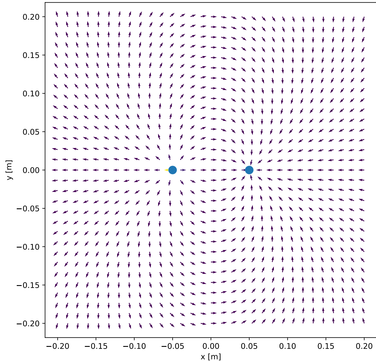
Electric Field Generated by Point Charges
