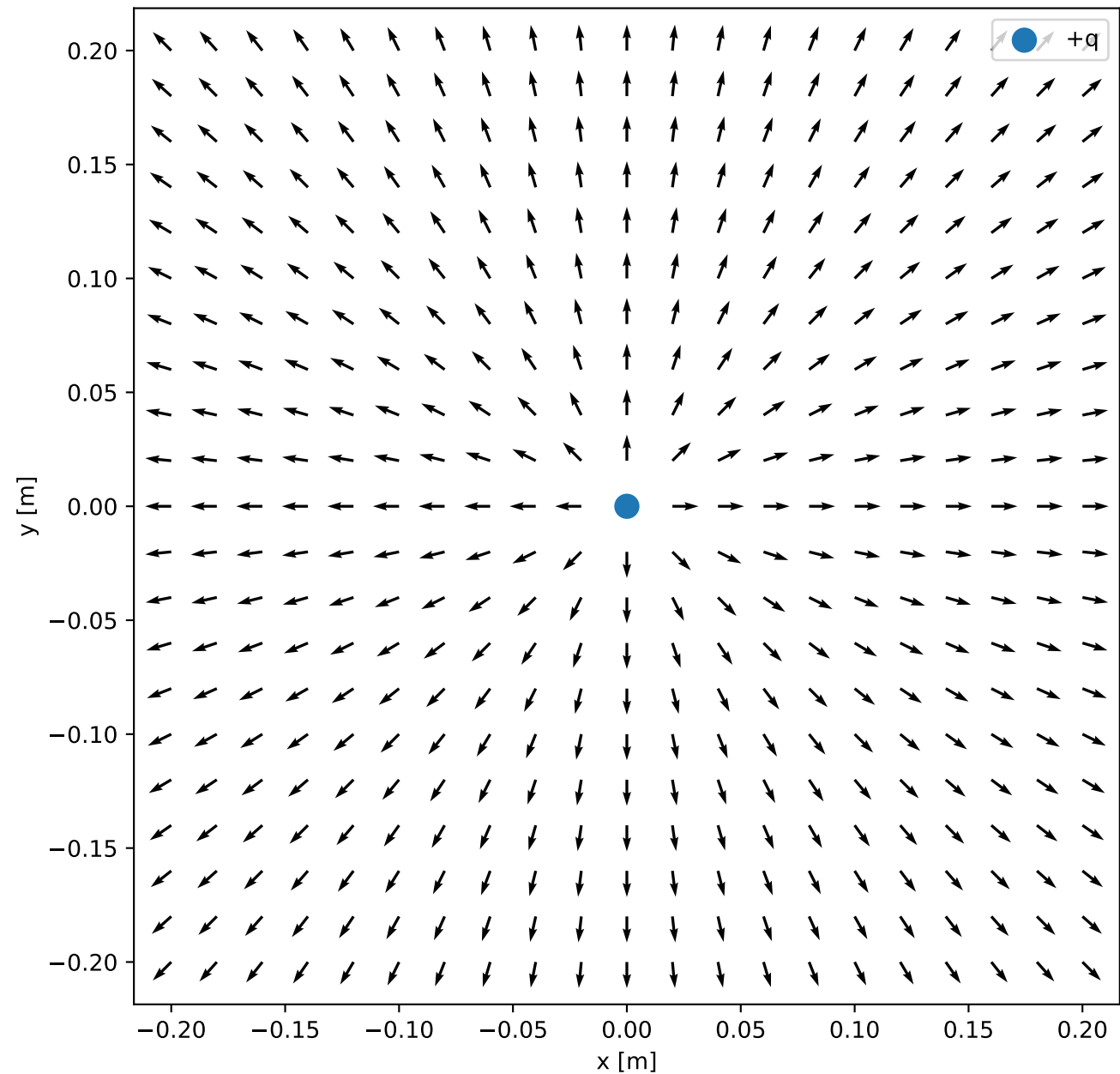
Electric Field Reconstructed from the Potential
