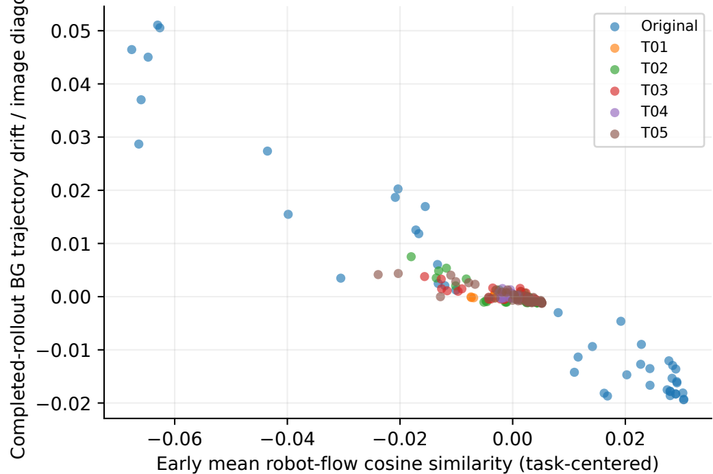
task_demeaned: \rho = -0.829 , 95% CI [-0.955, -0.568] n=270; early evaluations 0,4,8
