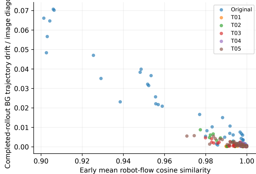
pooled: \rho = -0.730 , 95% CI [-0.857, -0.515] n=270; early evaluations 0,4,8
