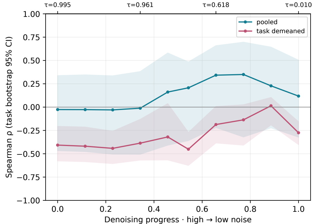
Final trajectory drift \leftrightarrow LOBO Action R^2 \cdot \text{linear}
