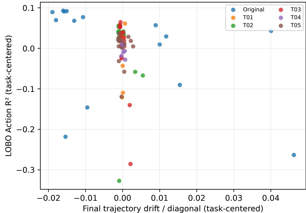
Early step 0 · 90 task/background pairs
