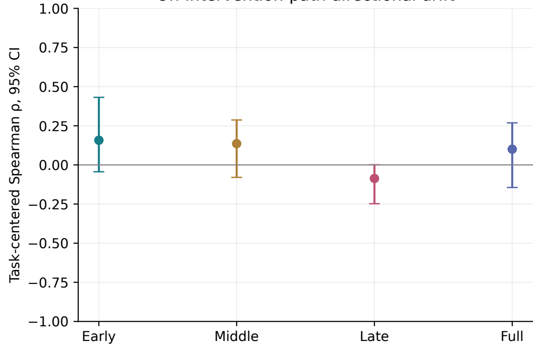
On-intervention-path directional drift
