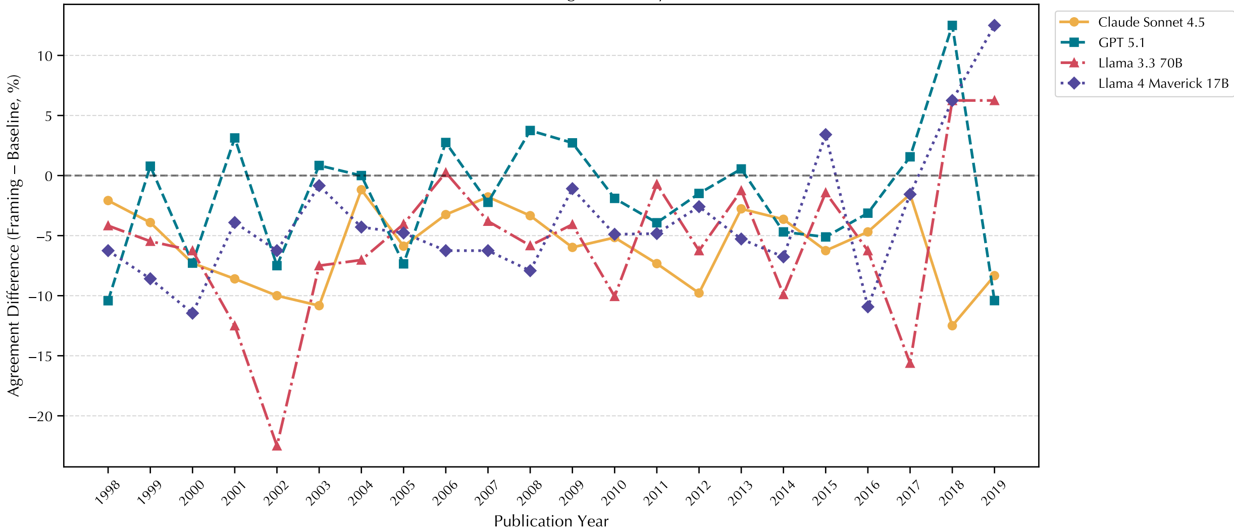
Evidence Direction Agreement by Year
